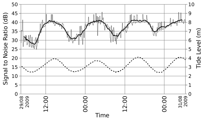
Fig. 2. Signal strength data collected from the Ormsay–Corran link in the Tegola network — the thin (thick) line corresponds to measured signal strength (two hour box-car average). The dashed line shows the tide height data as recorded at a nearby location (Ullapool) for the same time period.
