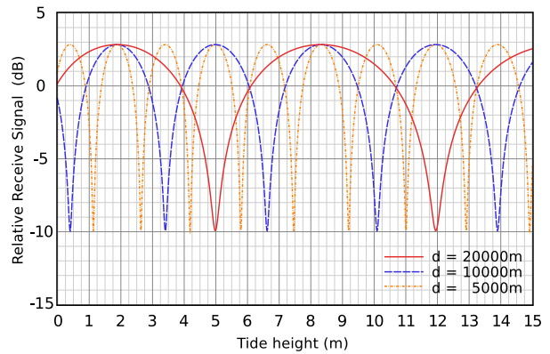
Fig. 4. Relative received signal strength vs. tidal height for links with both antennas 50m above sea level calculated using the geometric model with three link lengths. The reflection coefficient is 0.9. The frequency of operation is 5.180GHz (at 2.4GHz the null spacing would approximately double). Atmospheric effects and earth curvature are neglected.
