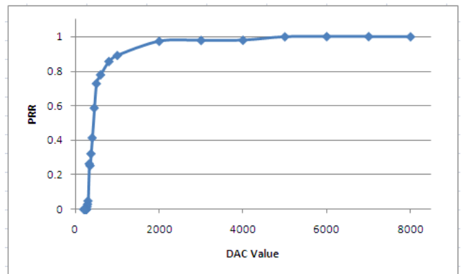
Fig.8 PRR for OFDM with QPSK modulation with 512 FFT bin
