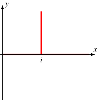
Standardbasis
