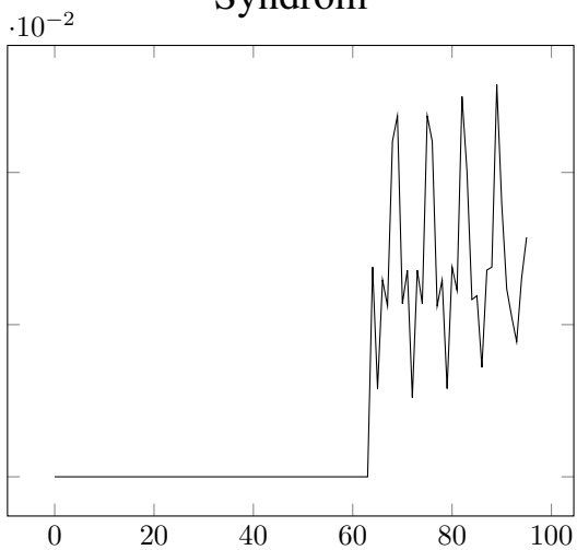
Syndrom
