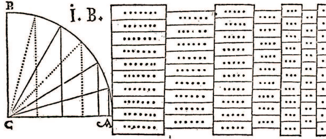
Figure 1: Fig. 1. Ursus's diagram ( Fundamentum astronomicum , fol. C1r)
