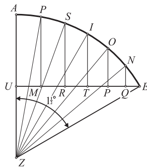
Figure 2: Fig. 2. Bürge's diagram for calculating \sin 1^\circ ( Fundamentum Astronomiae , fol. 32r)
